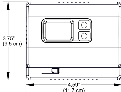
Horizontal design
